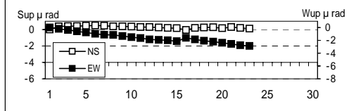
Ground Tilt at the point KOMA (Point KOMA : SWW 3.5km from the summit)
