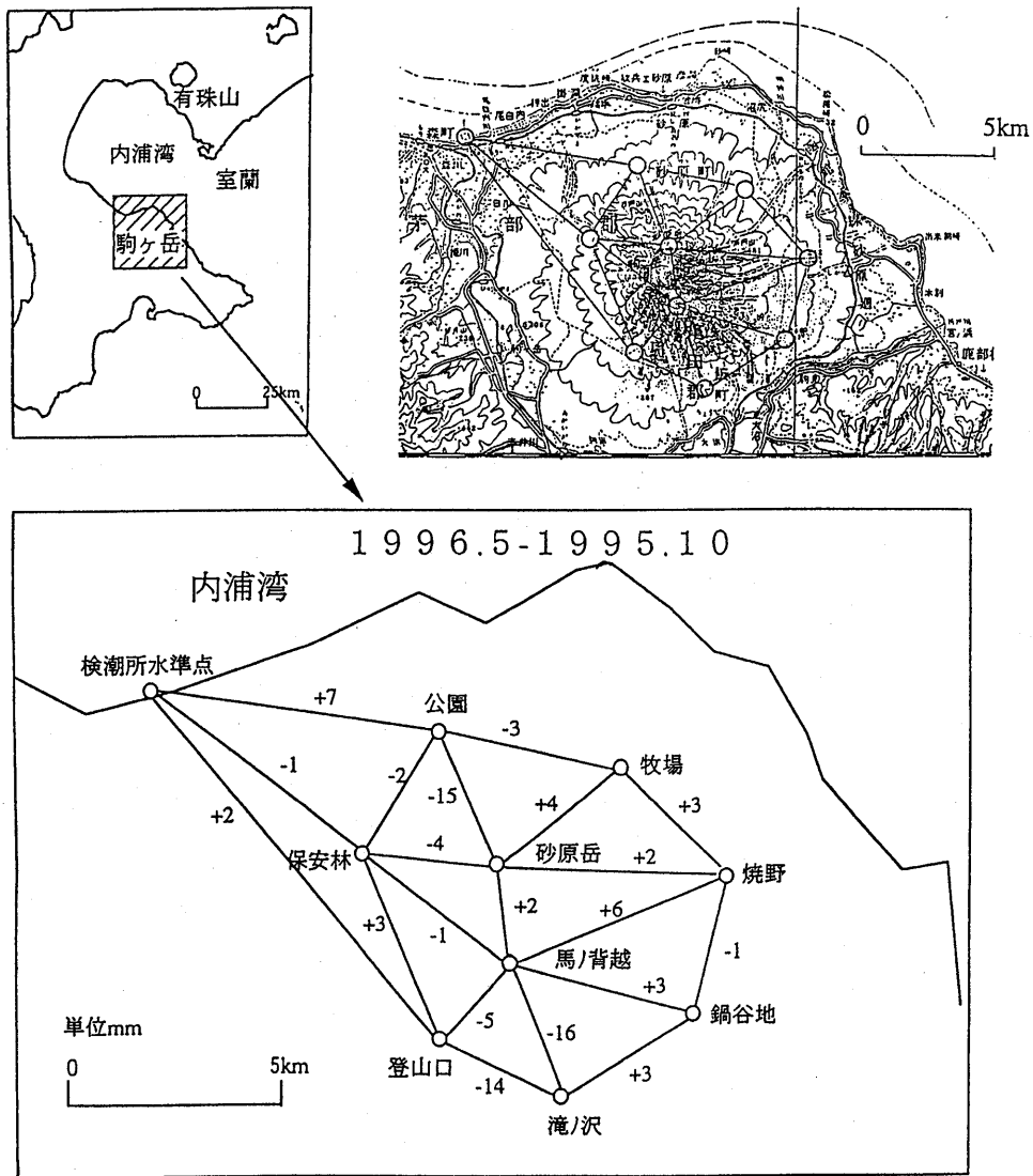
第 1 図 駒ヶ岳地方高度基準点測量結果 (標石間斜距離変化) Fig. 1 Results of the Advanced Geodetic Survey in the Komagatake area : line length changes between crustal deformation observation sites.
