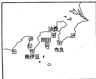
第 1 図 岡田・油壺・布良各験潮場間の月平均潮位差 Fig. 1 Differences in monthly mean sea level between Okada, Aburatsubo and Mera tidal stations.
