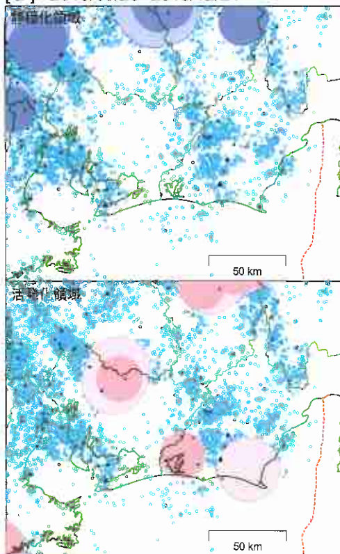
[2] 2015/09/26--2015/12/24
