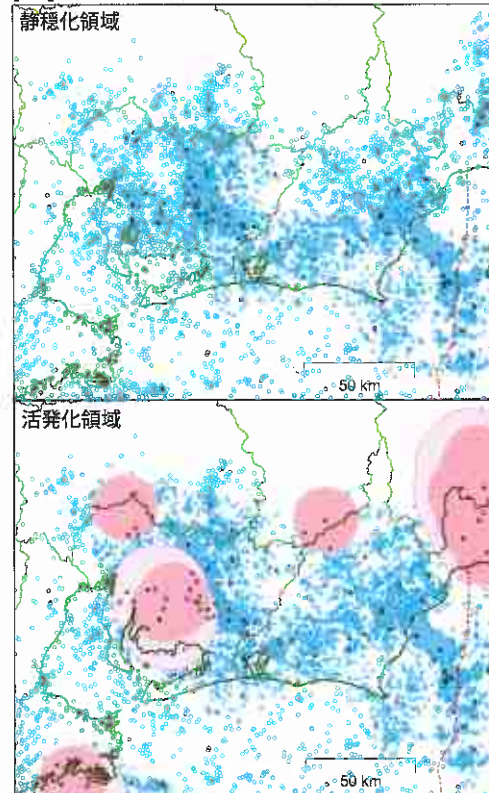
[ 1 ] 2015/06/28–2015/09/25
