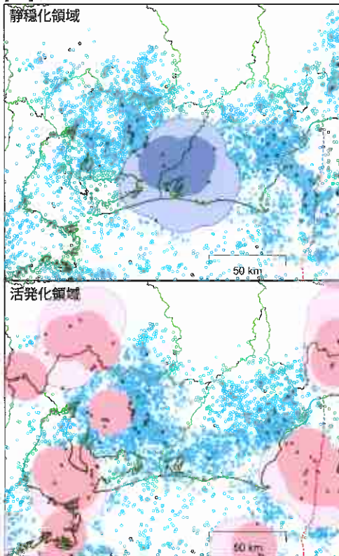
[ 2 ] 2015/09/26–2015/12/24
