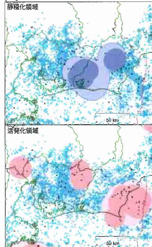
[ 3 ] 2015/12/25–2016/03/23
