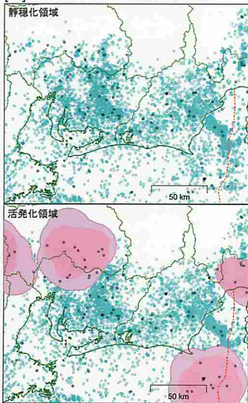
[ 2 ] 2014/07/26–2014/10/23
