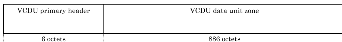
Figure 8-2 VCDU structure
