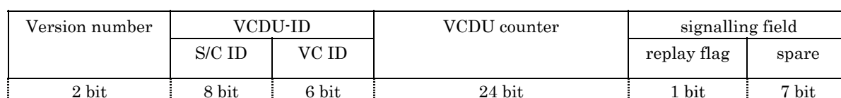
Figure 8-3 VCDU Primary Header
