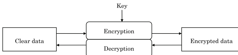
Figure 5-9 Encryption Principle
