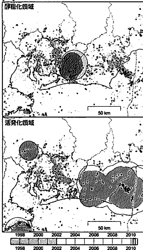
[2] 2010/03/27–2010/06/24
