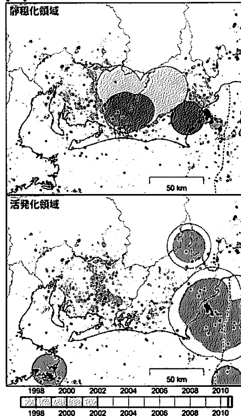
[3] 2010/06/25–2010/09/22
