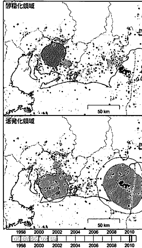
[1] 2009/12/27–2010/03/26
