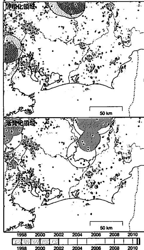
[3] 2010/06/25–2010/09/22
