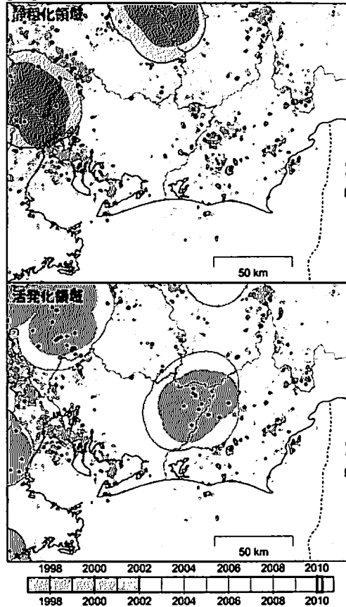
[1] 2009/12/27–2010/03/26
