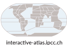
interactive-atlas.ipcc.ch
