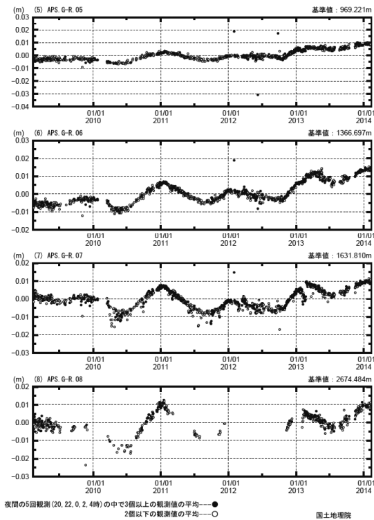
第4図 伊豆大島の光波測距観測結果(上段左：観測点配置図、上段右・下段左右：連続観測結果) Fig.4 Results of optical distance measurement observation around Izu-Oshima Volcano. (upper left) Location map of observation sites, (upper right and lower) Time series of optical distance measurement results from February 2009 to February 2014.
