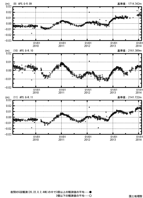
第4図 伊豆大島の光波測距観測結果(上段左：観測点配置図、上段右・下段左右：連続観測結果) Fig.4 Results of optical distance measurement observation around Izu-Oshima Volcano. (upper left) Location map of observation sites, (upper right and lower) Time series of optical distance measurement results from February 2009 to February 2014.
