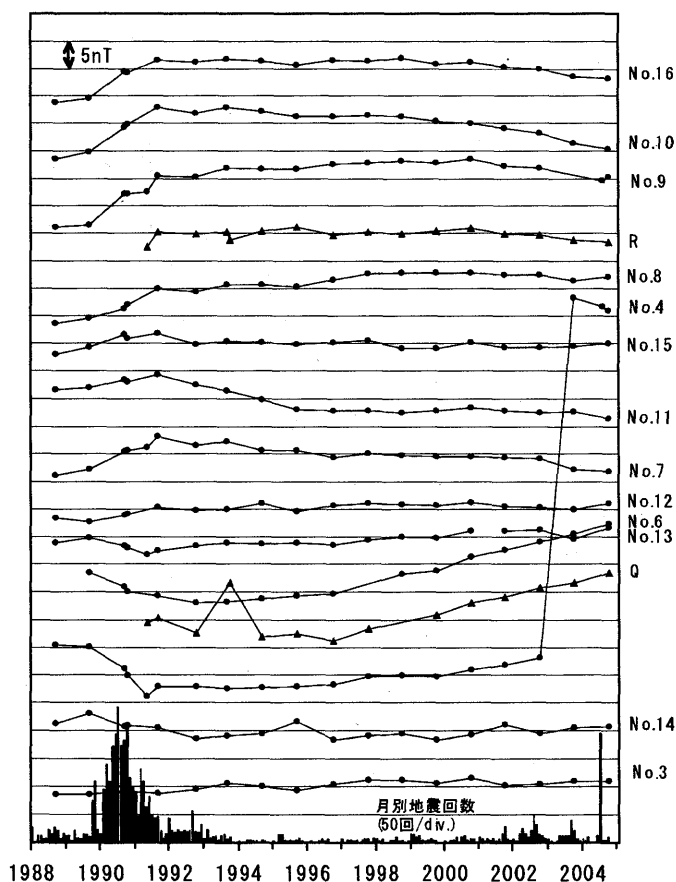
Fig.1 Location of continuous (solid square) and repeated (solid circle) observation stations of the geomagnetic total intensity.
