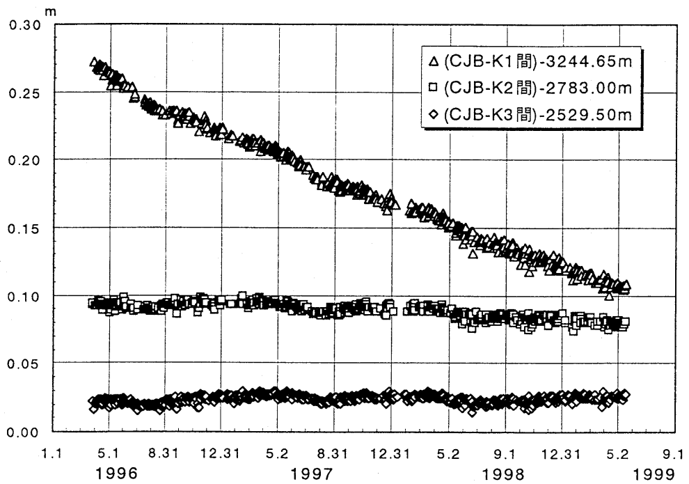
第2図 長者原-K1-3の光波測距結果。夕方の方のデータのみを示した。 Fig.2 Change in slope distances between Chojabaru and K1 to K3 using automatic EDM system. Selected data in stable atmospheric condition in the evening are plotted. Add 3244.65, 2783.00, and 2529.50m for each line.
