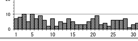
Number and Duration of Volcanic Tremors at the point STI1 located at 0.6km SSW from the summit
