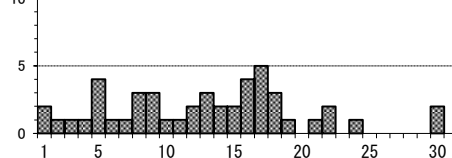
Number and Duration of Volcanic Tremors at the point SKRB located at 2.3km NW from Minamidake crater
