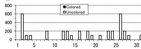
Maximum Plume Height (Showa crater)
