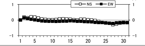
Ground Tilt at the point SETO located at 4.8km ESE from Minamidake crater
