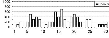
Maximum Plume Height
